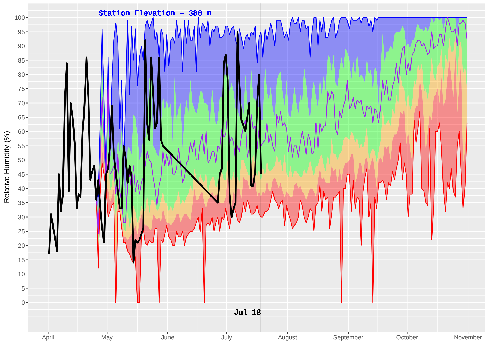
BELL-IRVING (432) : Historical (1986–2016) and Current (2018) Daily Relative Humidity
